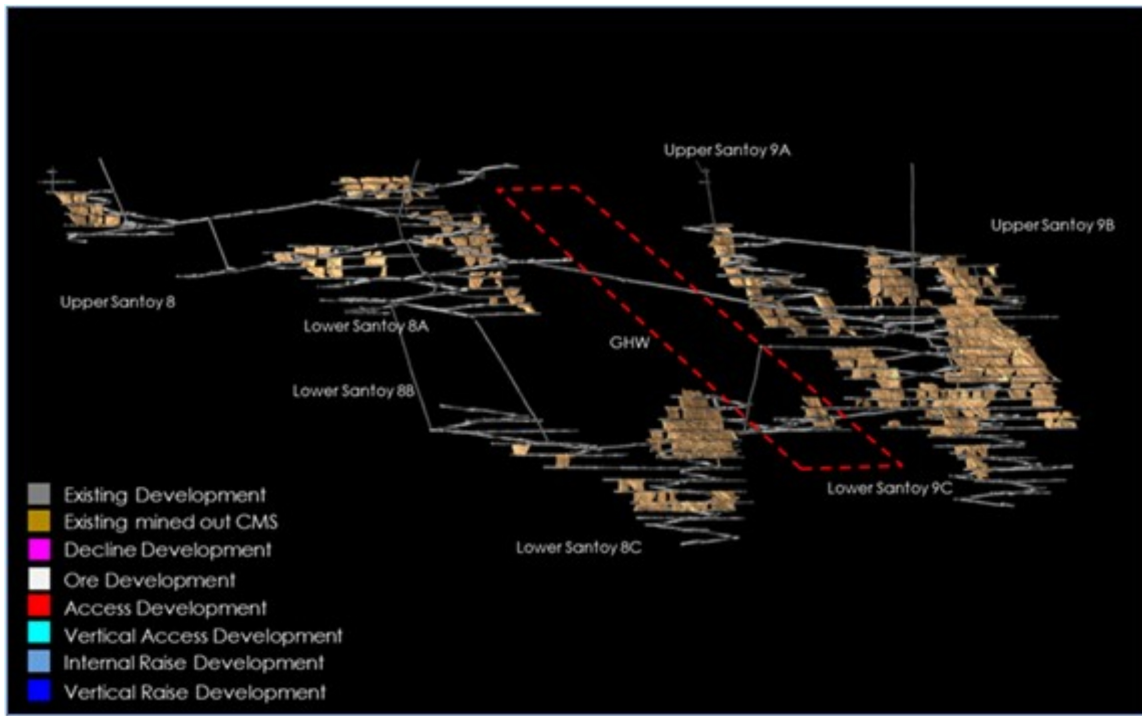
Figure 13.1 Santoy Mine – Existing Development
