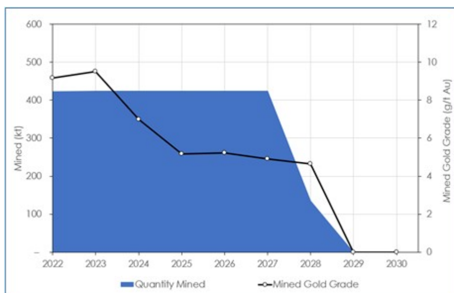
Figure 19.1 Production Plan Tonnage
