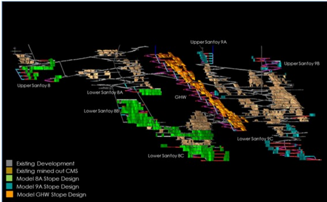
Figure 13.3 Santoy Mine – 2021 Life-of-Mine Stope Designs
