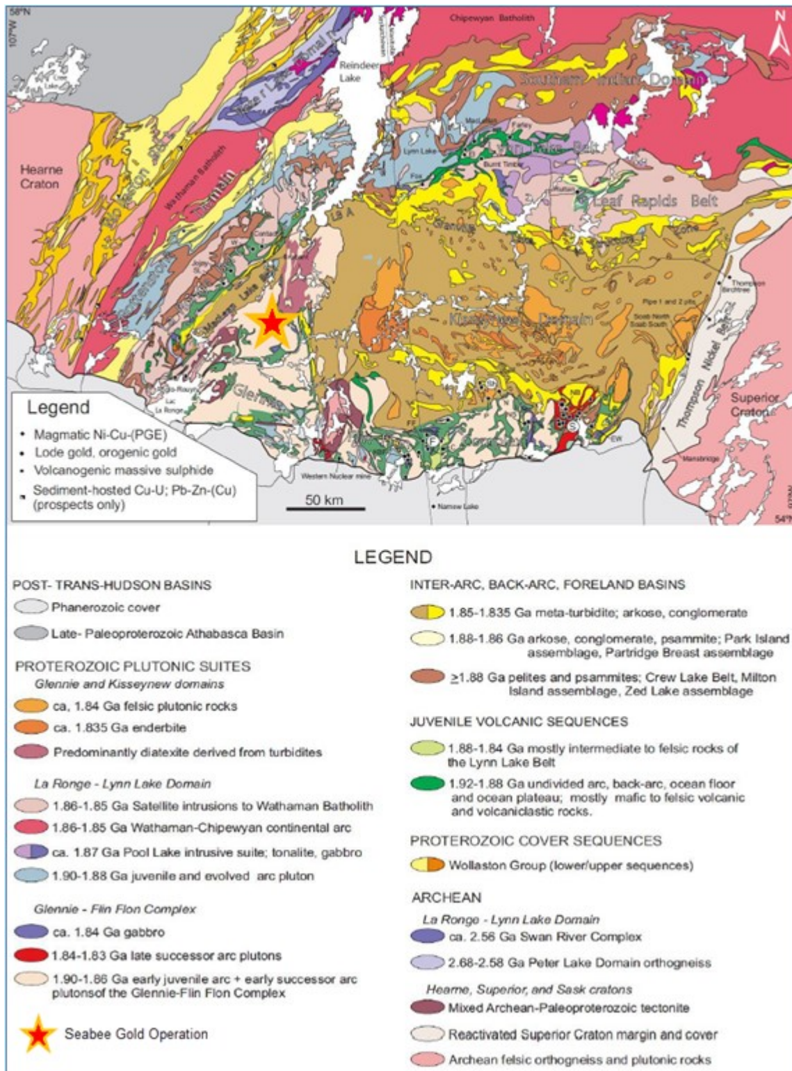
Figure 6.2 Regional Geology of the South-Western Trans-Hudson Orogen
