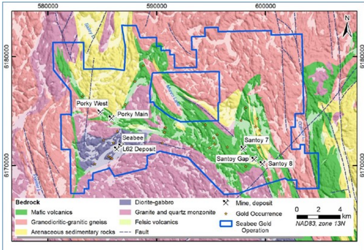
Figure 6.3 Local Geology Setting
