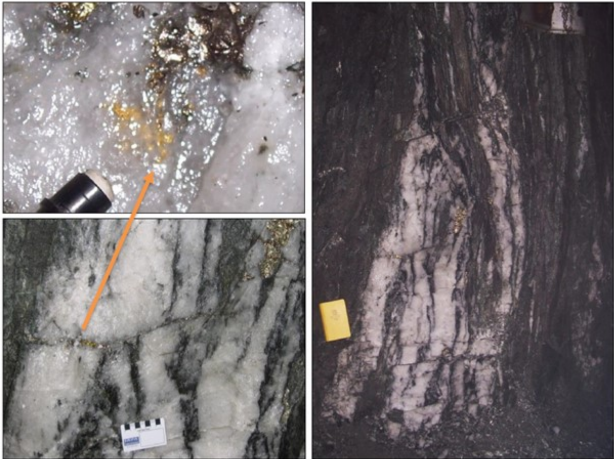
Figure 6.5 Typical Mineralisation Observed at the SGO
