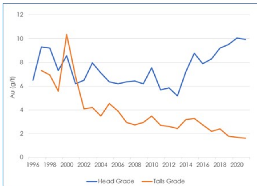
Figure 10.2 Historical Annual Head and Tailings Grade Trend
