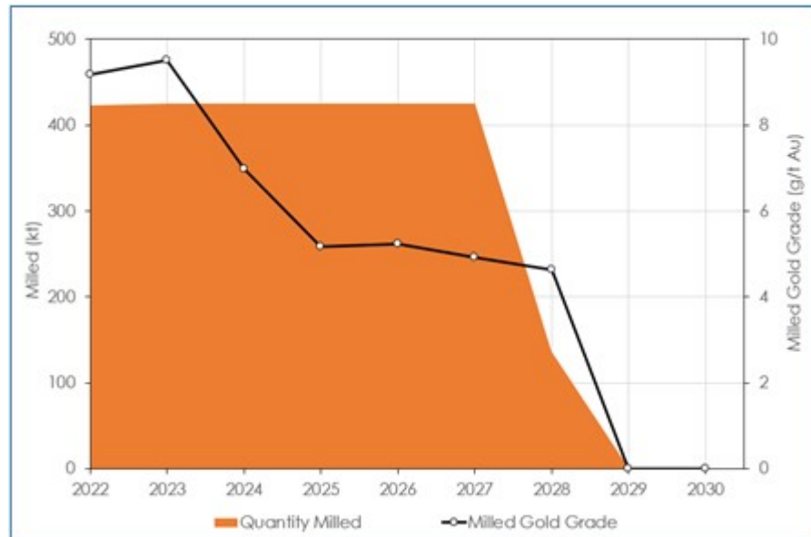
Figure 1.3 Process Feed Profile
