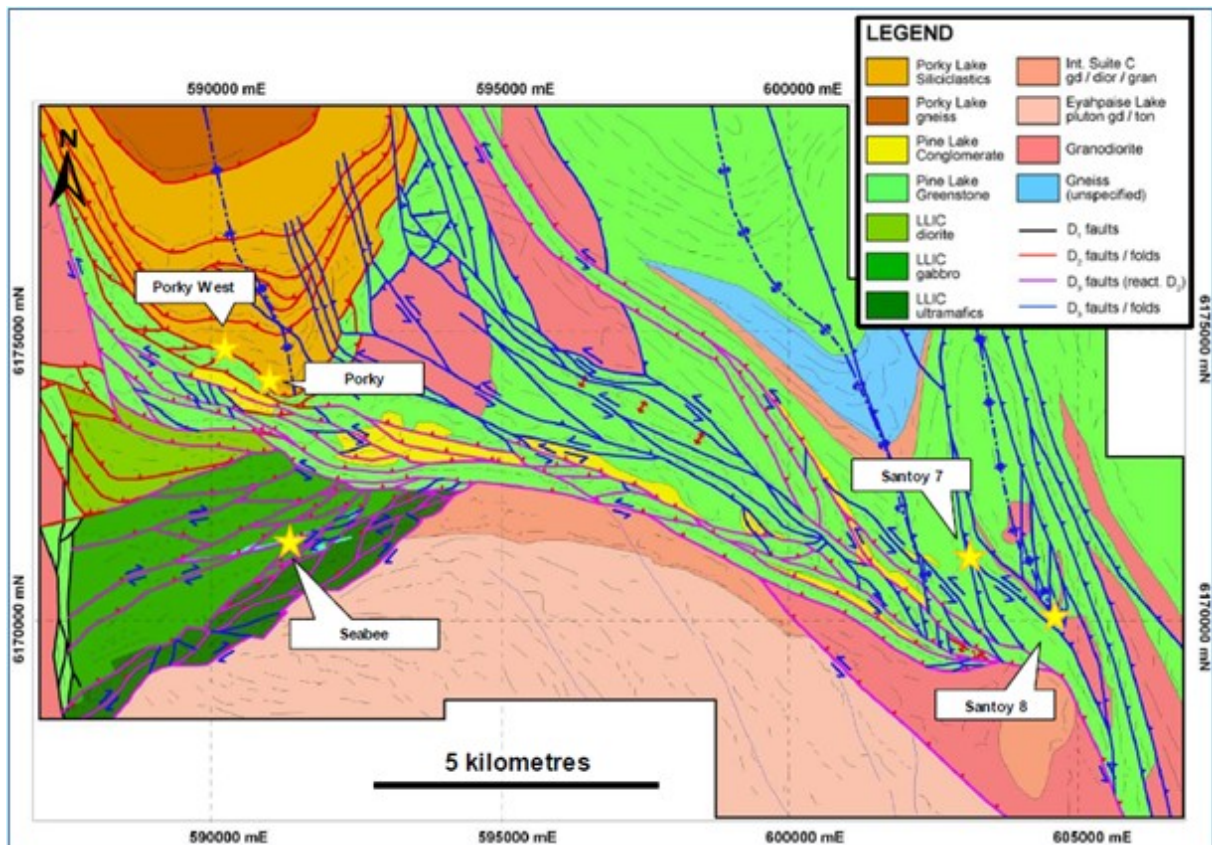
Figure 6.4 Integrated Structural Analysis of the SGO by SRK (2009) Based on Goldak's 2007 Aeromagnetic Survey
