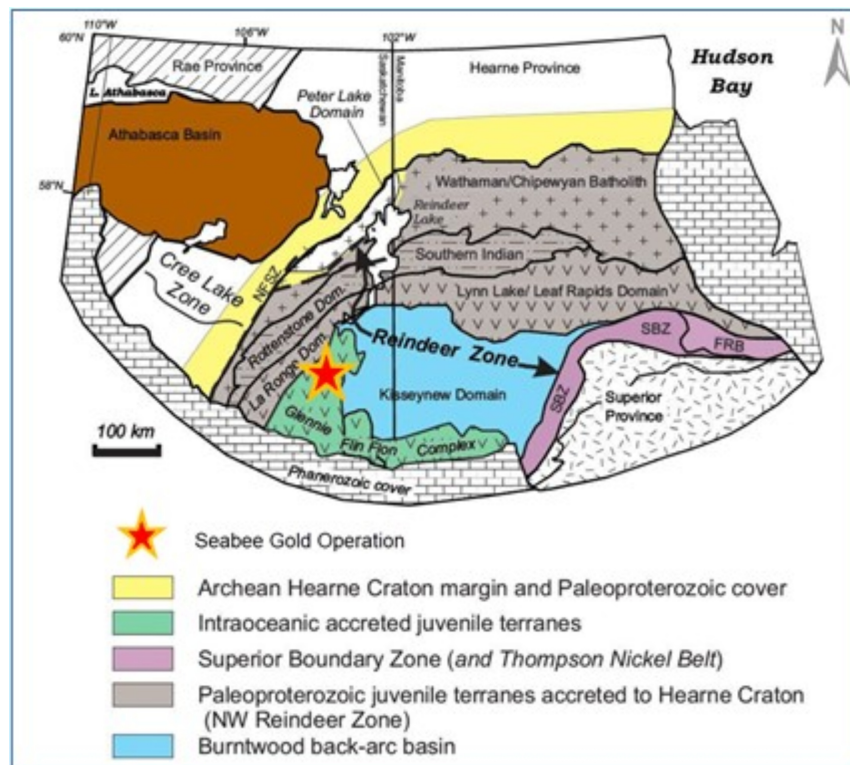
Figure 6.1 Cree Lake Zone and Reindeer Zone of the Trans-Hudson Orogen
