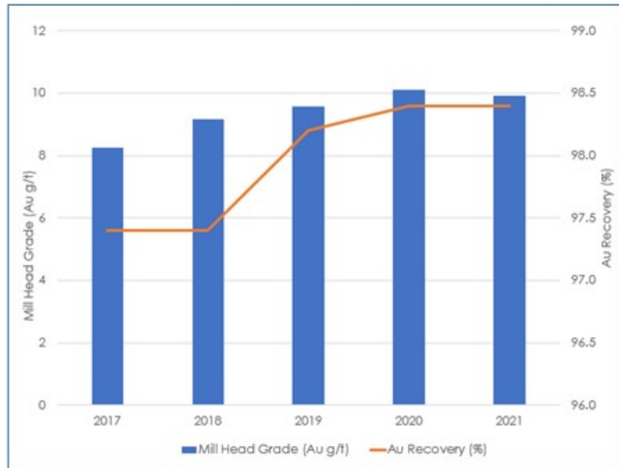
Figure 10.3 Mill Feed Grade and Gold Recovery 2017–2020
