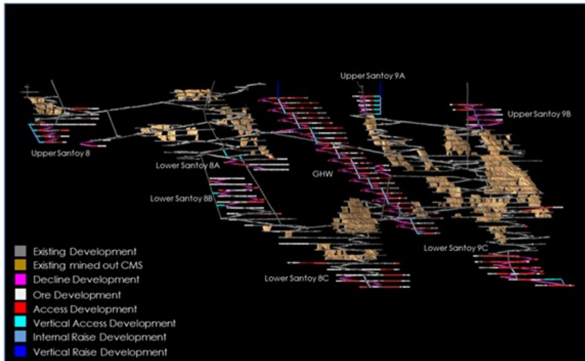
Figure 13.2 Santoy Mine – 2021 Life-of-Mine Development Design
