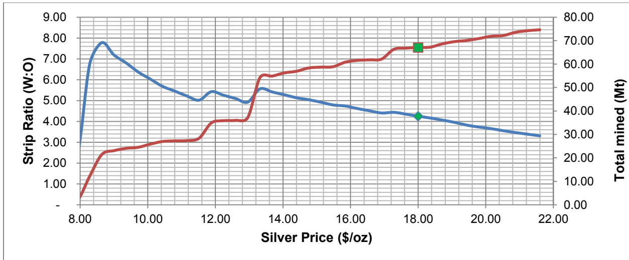
Figure 15-6: Total rock mined (red) and strip ratio (blue) for different silver prices
