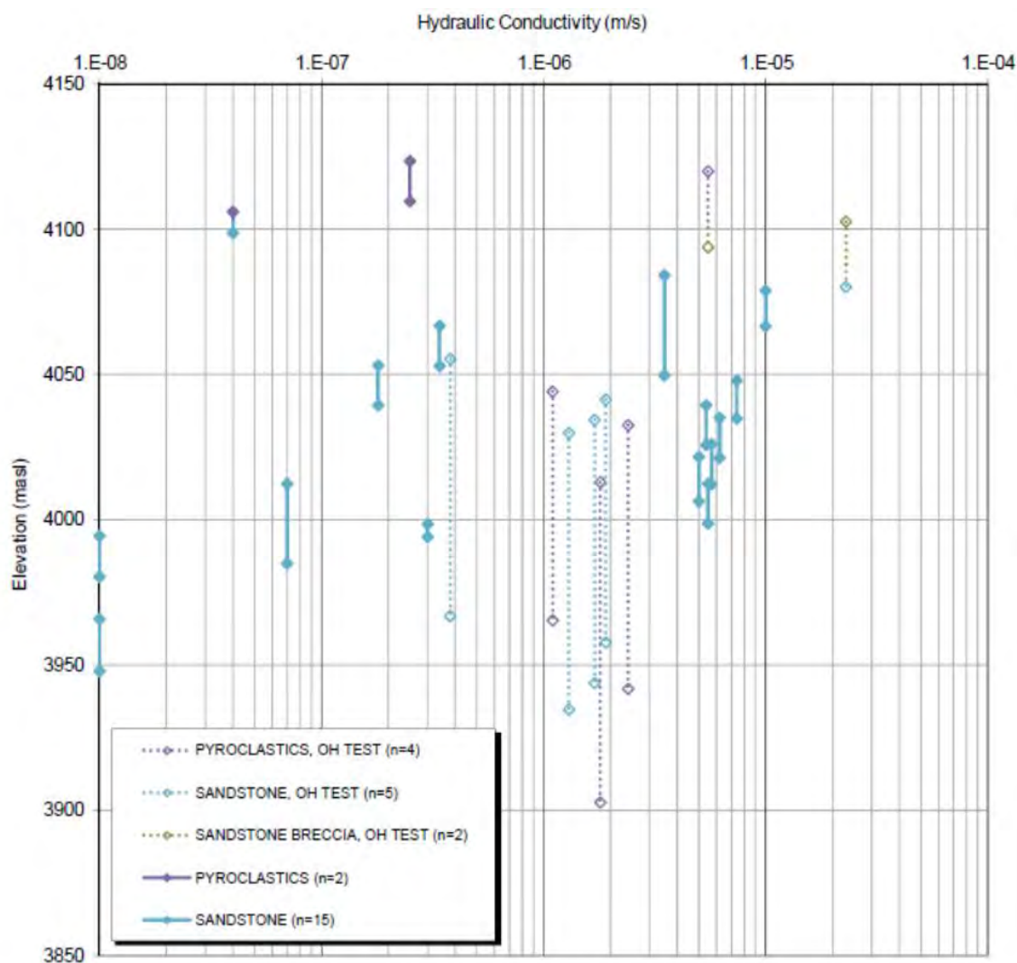
Figure 20-1: Response Test Hydraulic Conductivity by Lithology
