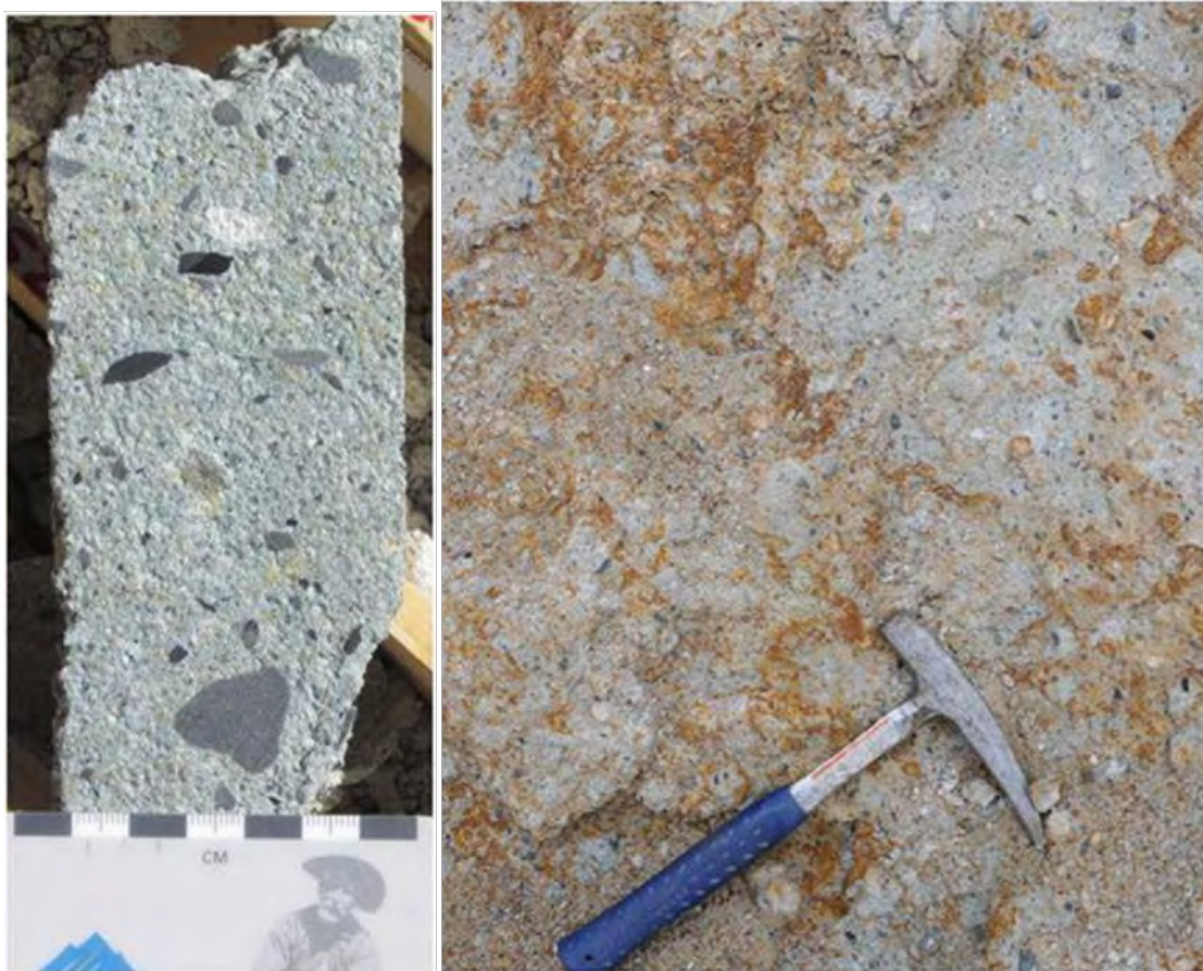
Figure 7-8: Typical Chinchillas Medium Grained Pyroclastic Breccia with Dacitic Volcanic Clasts Dominant and Secondary Dark Grey Clasts of Basement Sandstone and Pelite. (Golden Arrow, 2013)
