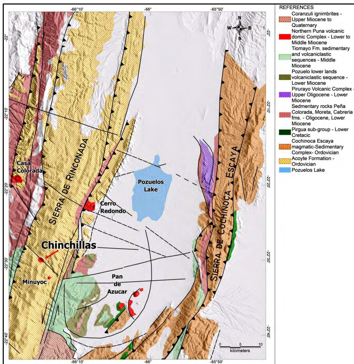
Figure 7-3: Map Showing Tertiary Volcanism from Mega Caldera Complexes Near the Chinchillas Deposit. (Main structures and trends are also shown.) (Modified from Caffé 2002)
