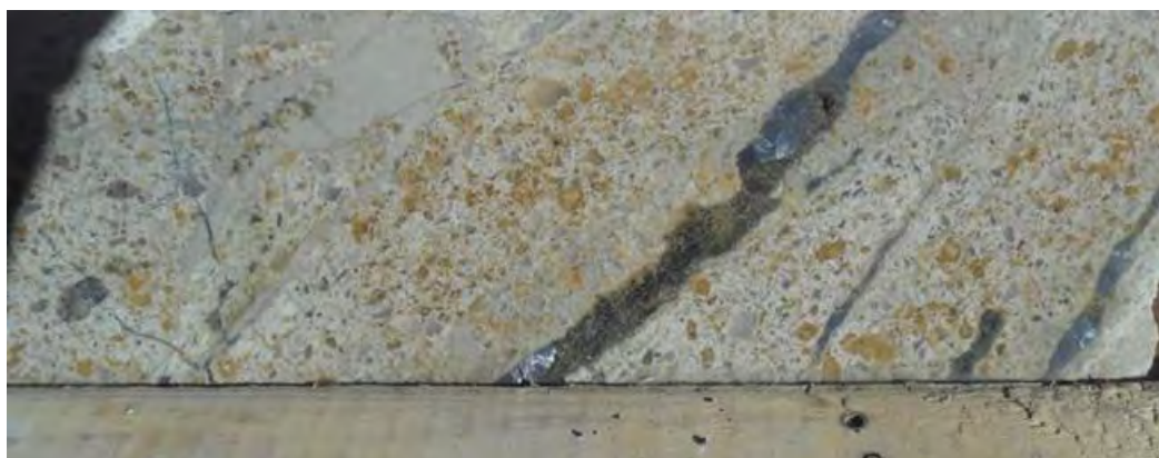
Figure 7-19: Galena-Ag Veinlets in Dacite. (Golden Arrow, 2014)
