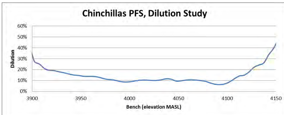
Figure 15-5: Dilution by Benches at Chinchillas Pit
